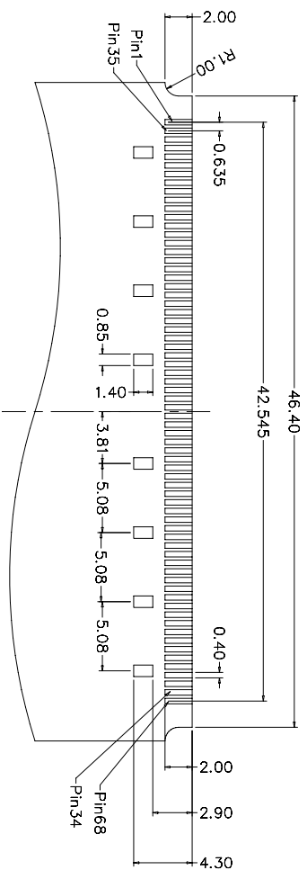
Recommended PCB Layout
